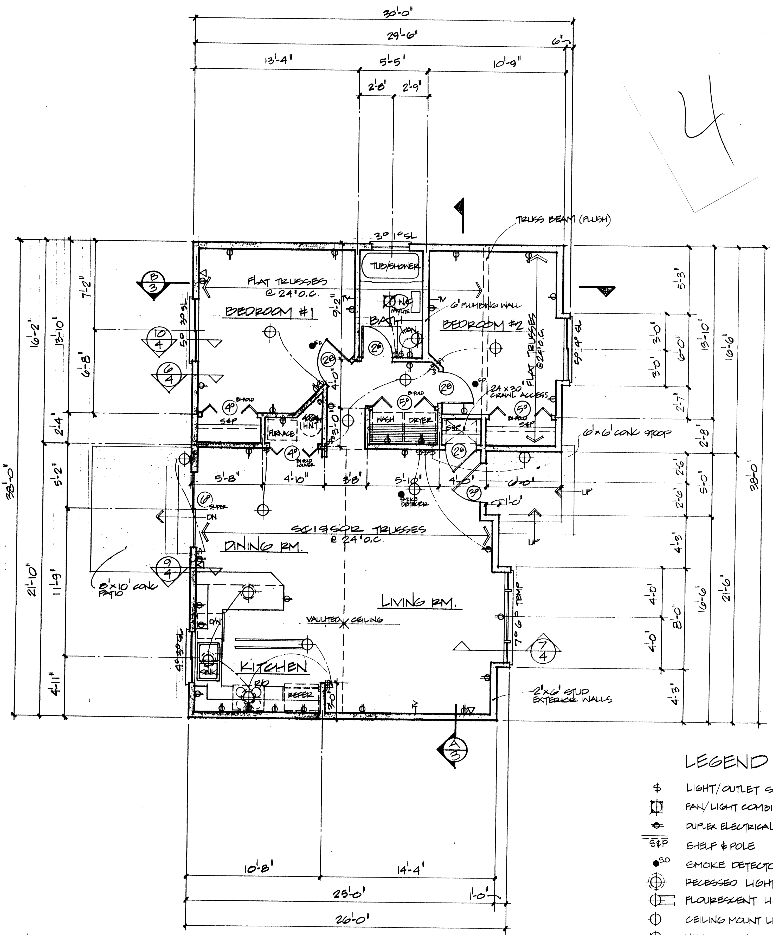
MAIN FLOOR PLAN 1/4" = 1'-0"
