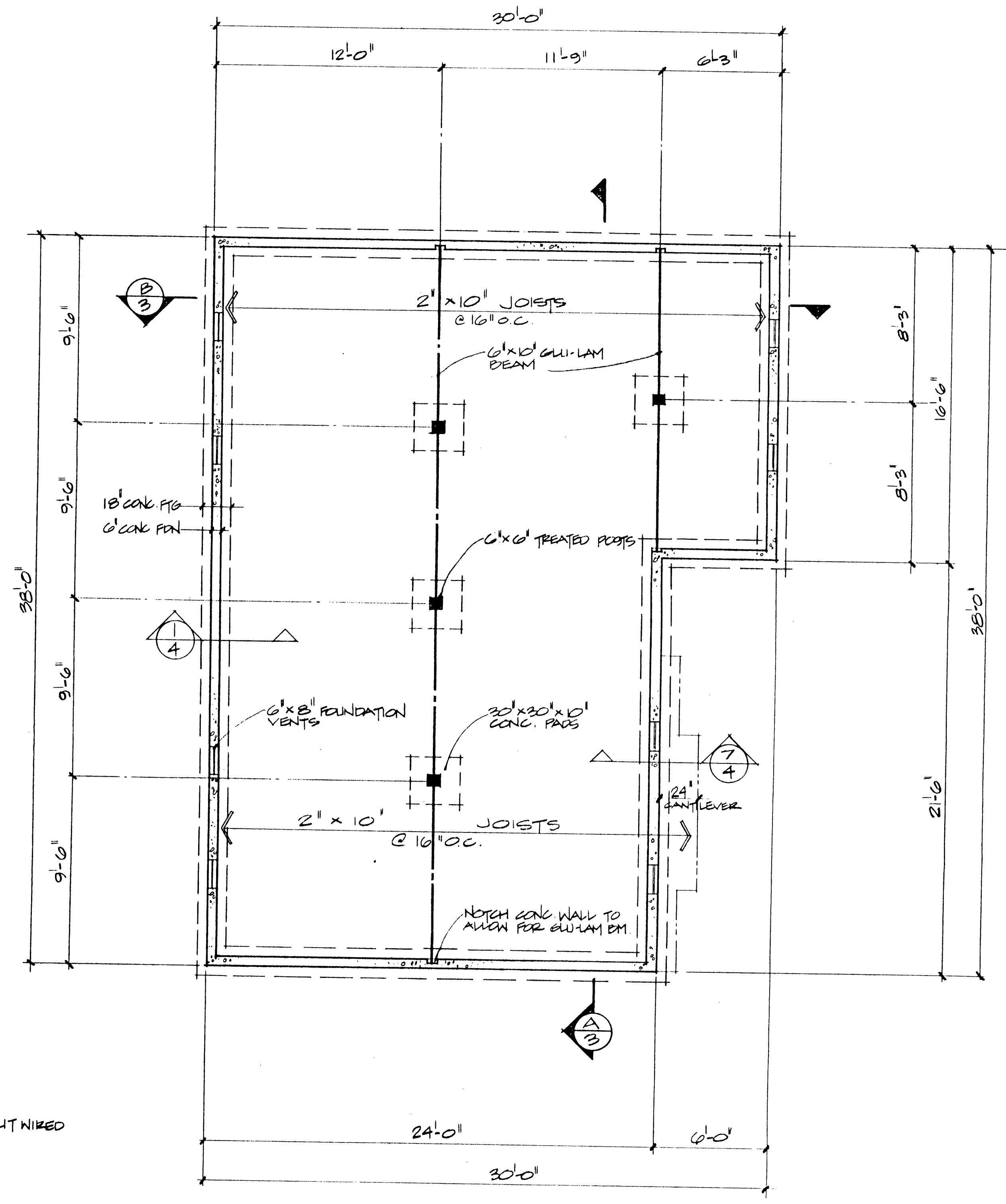
FOUNDATION PLAN 1/4" = 1'-0"
